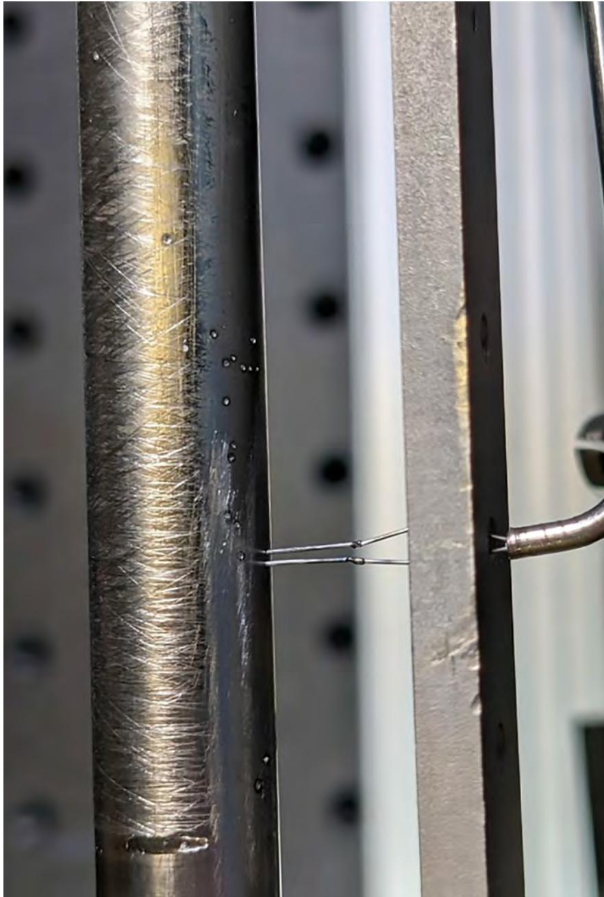
Figure 2. Cladding thermocouple weld
