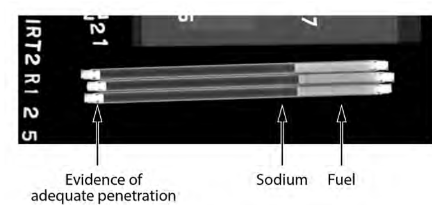
Figure 3. Overall radiography of the IRT-2 irradiation test
