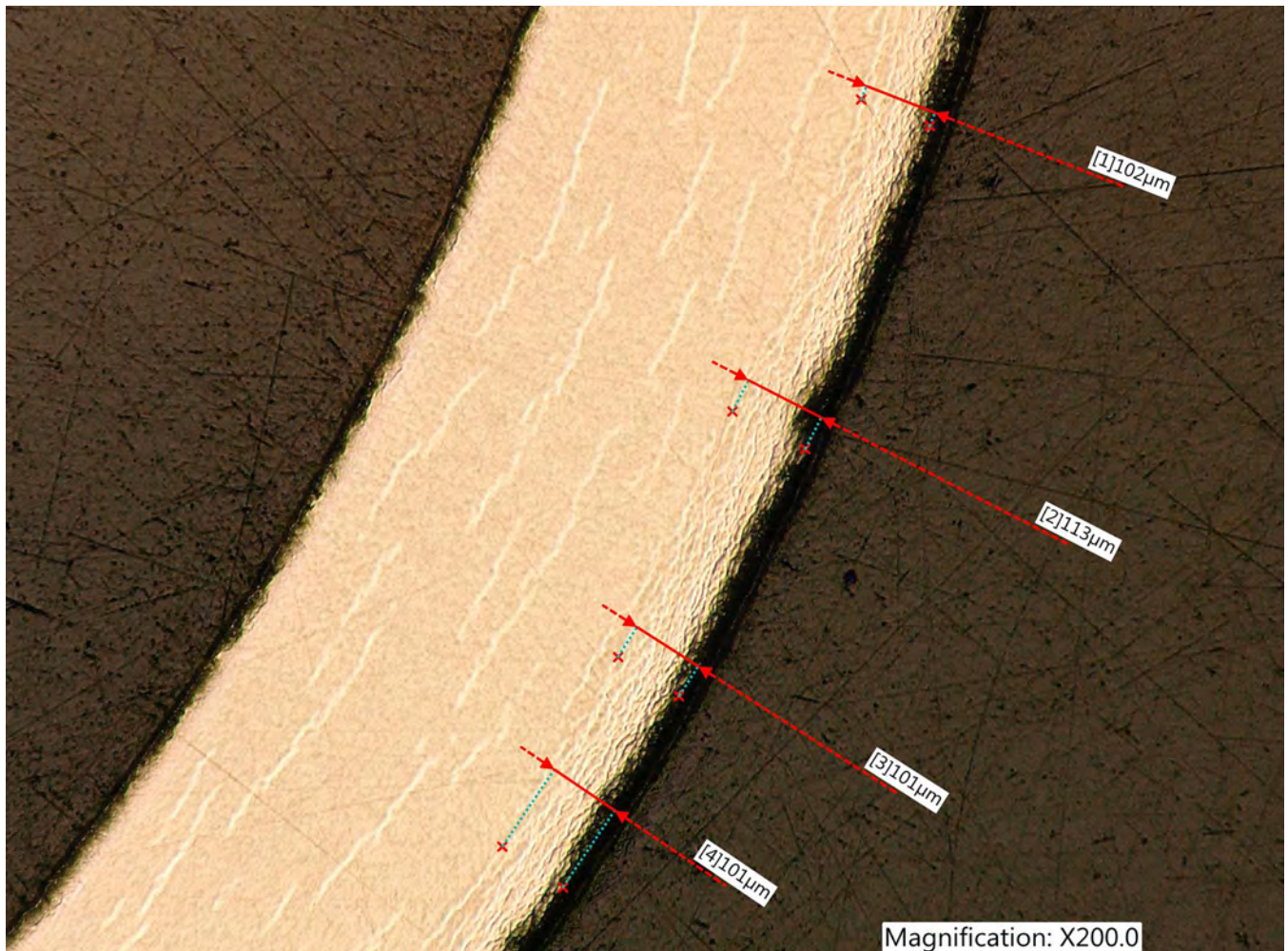
Figure 3. Hydrided cladding with 100 \mu\text{m} rim
