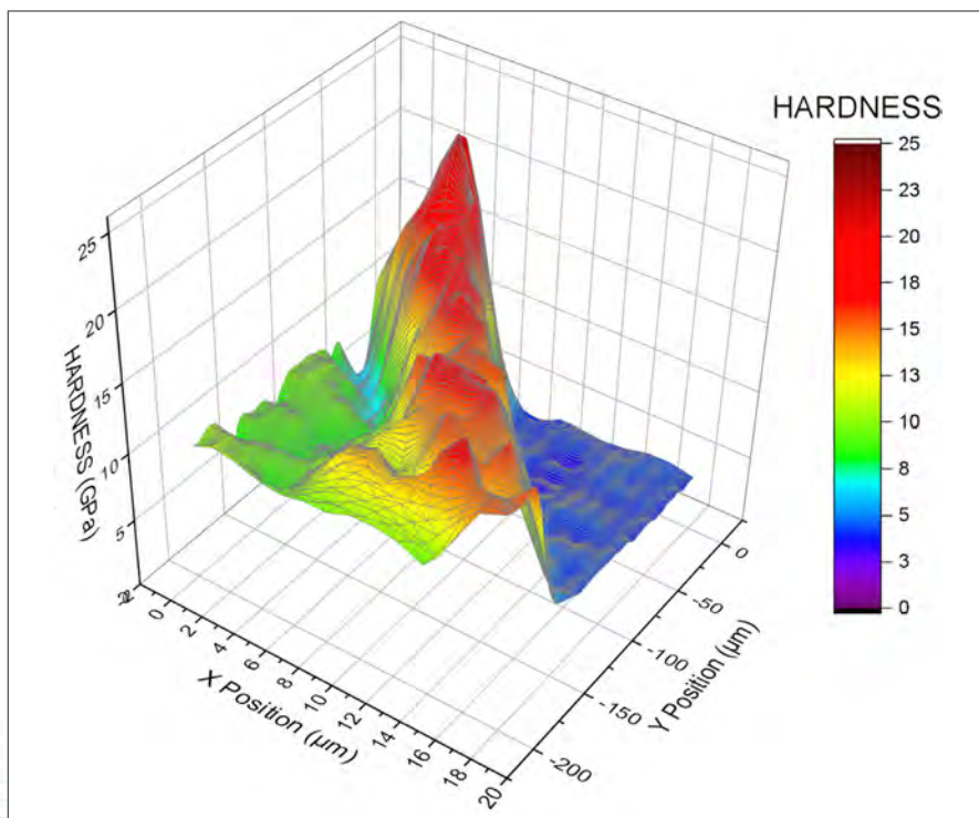
Figure 2. Nanoindentation of Cr-coating on Zry-2
