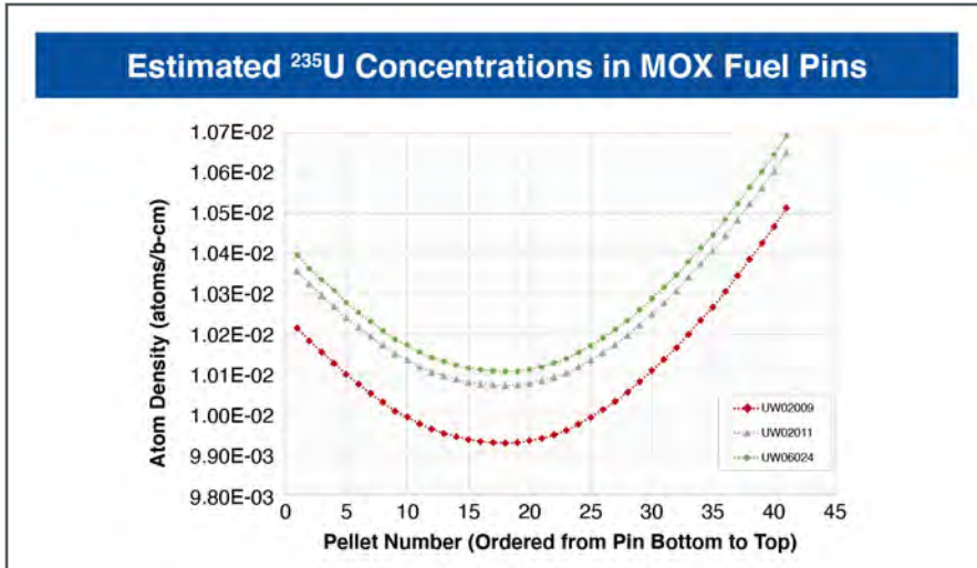
Figure 3. THOR-MOXTOP experiment specimens: (Top) predicted axial ^{235}\text{U} concentration in pins, (Middle) Recovered neutron radiograph showing pin UW02009, (Bottom) photo of test pin UW02009 in hot cell during retrieval from storage facility.
