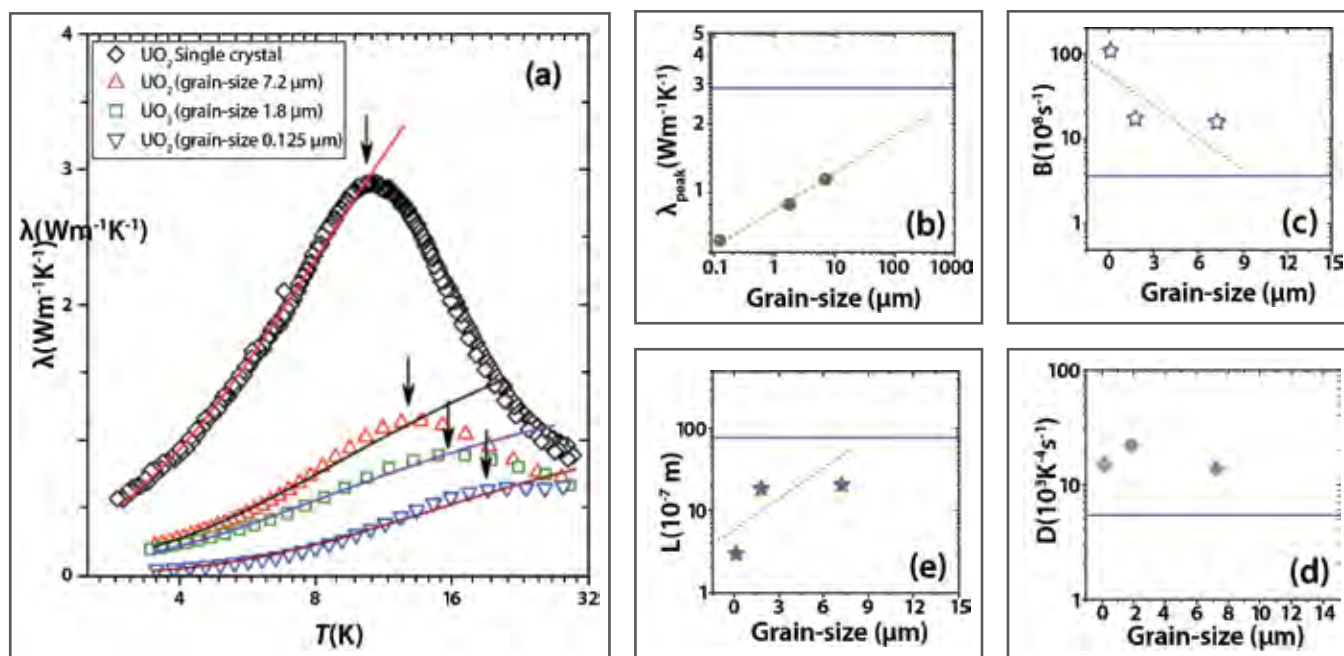
Figure 2. (a) The low temperature thermal conductivity of UO_2 samples. The solid lines represent the least-square fits of the Callaway model to the experimental data; The grain-size dependence (obtained from the Callaway model) of the low-temperature thermal conductivity peak (b), parameters B (c), D (d), and the mean free path of phonons L (e). The corresponding values for the UO_2 single-crystal are displayed as a horizontal line in the relevant graphs. The dashed lines are guides to the eye.
