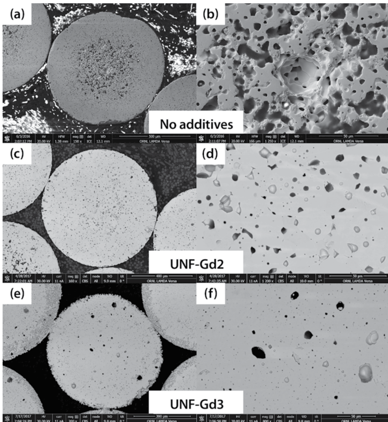
Figure 1. Typical microstructures of UN with no Gd (a-b), UN with Gd 0.025 heavy metal mole fraction (c-d), and UN with Gd 0.125 heavy metal mole fraction (e-f). High-resolution micrographs in each case was obtained focusing on the center of the samples.
