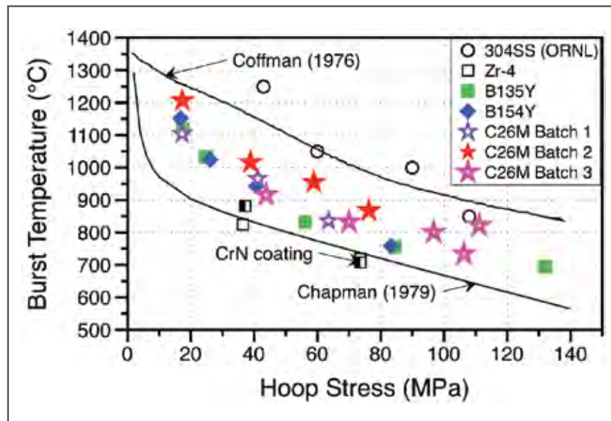
Figure 2: Burst temperature as a function of engineering hoop stress for various cladding materials examined in the SATS (data points from this year and prior years) alongside empirical correlations (lines) from the literature for Zr-alloys and type 304 stainless steel (SS).
