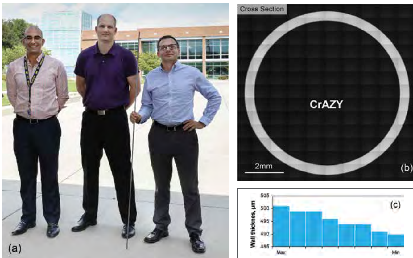
Figure 1: a) CrAZY ODS FeCrAl tube, b) Cross-section of the tube, c) Wall thickness measurements showing the excellent dimension tolerance
