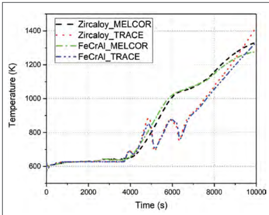
Figure 2. Comparison of MELCOR and TRACE prediction of peak cladding temperature during a station blackout scenario for a PWR benchmark problem with Zirc-4 and FeCrAl claddings.
