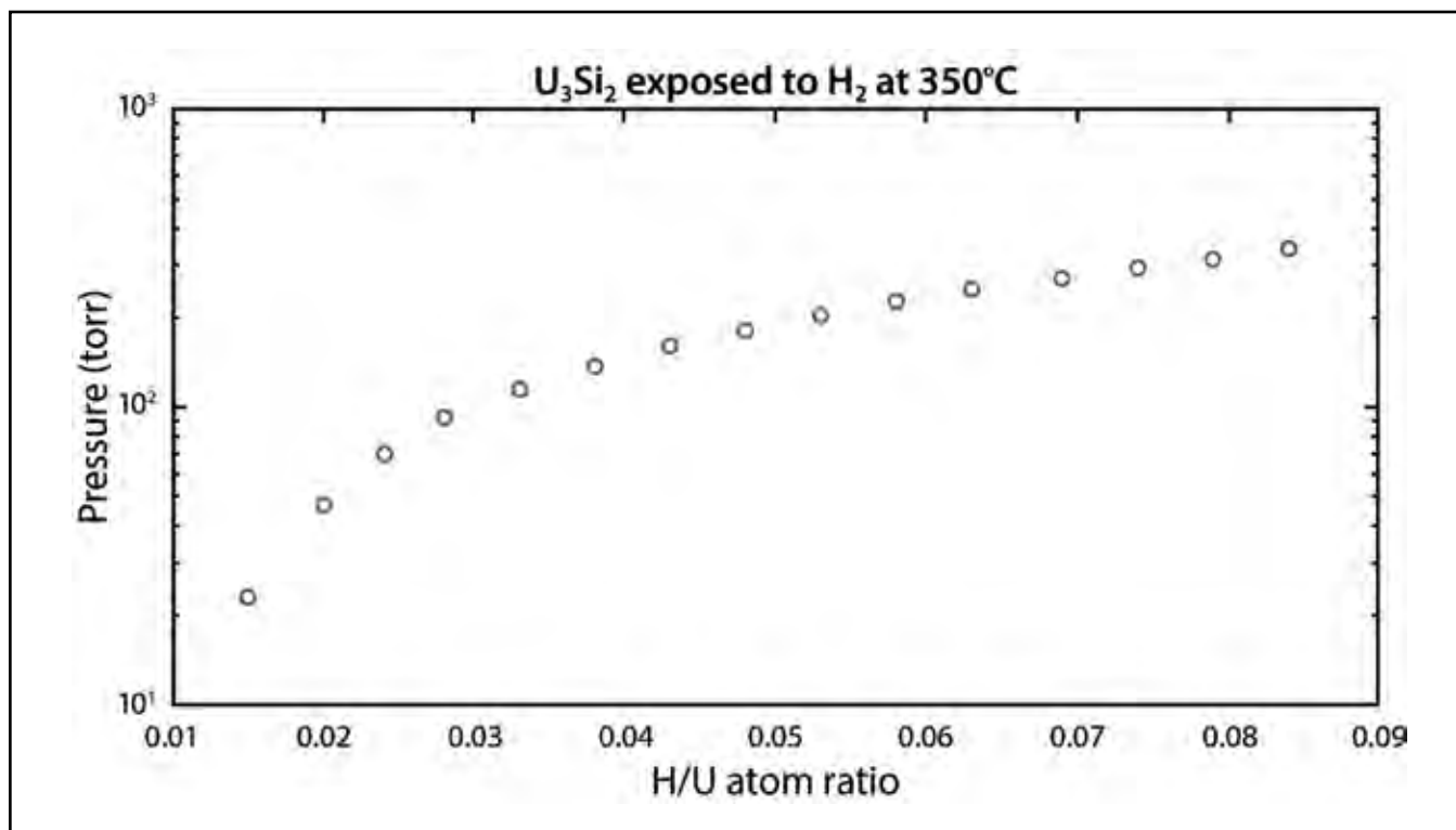
Figure 2: Pressure-composition-temperature isotherm for hydrogen absorption of \text{U}_3\text{Si}_2 at 350^\circ\text{C} . Hydriding was terminated at 320 torr of \text{H}_2 and absorbed hydrogen corresponding to a H/U ratio of 0.084.
