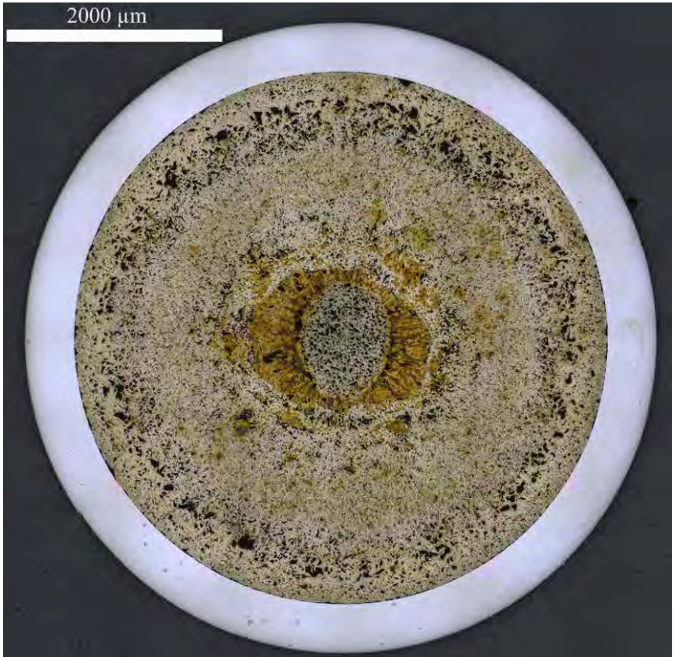
Figure 3. X501-G591 metallography near the axial mid-plane of the fuel slug
