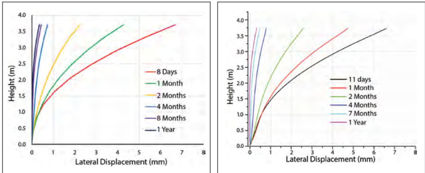
Figure 3. Plots comparing the lateral displacement magnitude predicted by BISON (left) and Abaqus (right).
