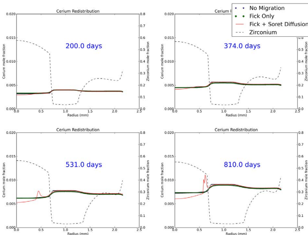
Figure 86. Snapshots of Modeled Cerium Production and Solid-state Migration. The burnup is roughly 3at.%, 5at.%, 7at.%, and 9at.% for the days shown. Number of days shown, begins from the first day of burning of the fuel and included days when the rod was not burning. The red solid line shows the best physical model for cerium solid state diffusion and barely deviates from the “no diffusion” case. Soret diffusion is the main driver of cerium solid-state migration and the most mobility exists for bcc \delta -cerium.
