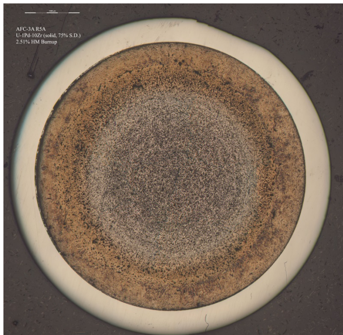
Figure 110. Optical microscopy of AFC-3A R5A possibly exhibiting the 2 zone Zr redistribution behavior typically observed in historic irradiations of U-10Zr fuel.
