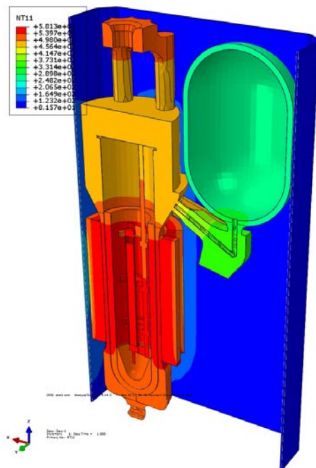
Figure 71. Thermal Finite Element Model Example.
