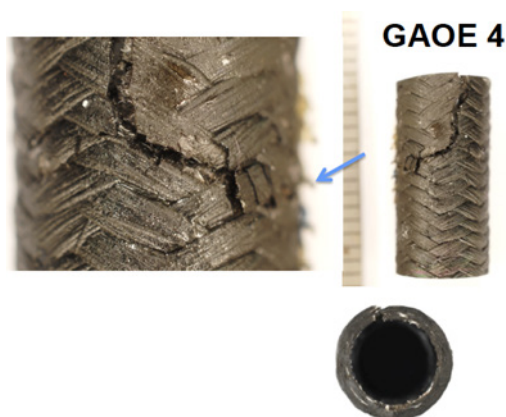
Figure 9. Oxidized burst testing of General Atomics Open Ended (GAOE) sample number 4.
