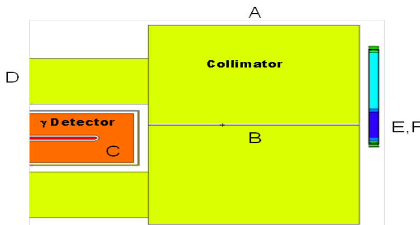
Figure 116. A cross section of the MCNP6 modeled system geometry with references to the optimization parameters (A-F).
