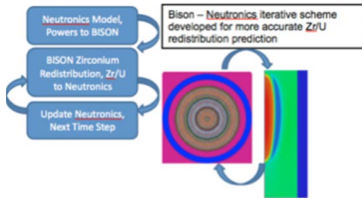
Figure 79. The sketch of Bison-neutronics coupling.
