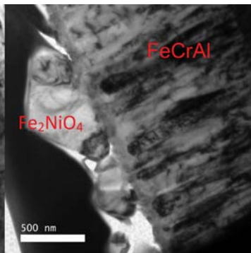
Figure 12. TEM image of FeCrAl/ \text{NiFe}_2\text{O}_4 spinel interface after 10 days exposure in the simulated BWR-NWC environment.
