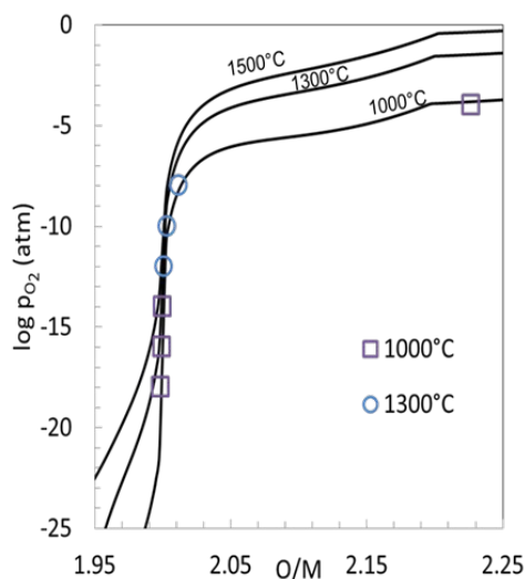
Figure 5. Thermogravimetric measurements of oxygen potential as a function of O/M ratio for \text{U}_{0.90}\text{Pr}_{0.10}\text{O}_{2\pm x} performed at ORNL.
