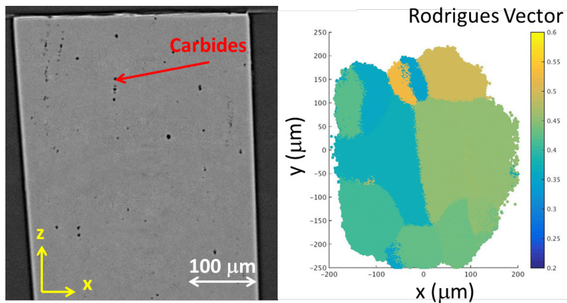
Figure 119. (a) (Left) Absorption tomography slice of an x-z plane in an austenitic steel showing metal carbide precipitates; (b) (Right) High-energy diffraction microscopy results of the same austenitic steel indicating grain morphologies and orientations through the x-y plane of a 2-μm slice.
