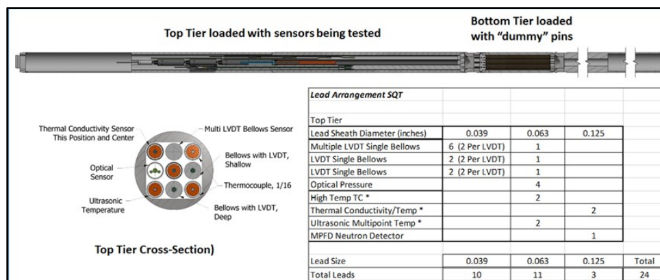
Figure 68. ATF-2 SQ Test Train Design
