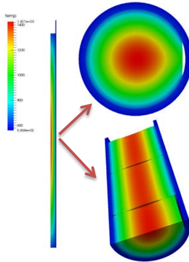
Figure 75. BISON simulation of the effects caused by a missing pellet surface.
