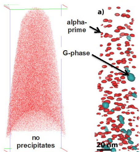
Figure 106. Alpha-prime and G-phase formation in HT-9 after irradiation at 375°C.
