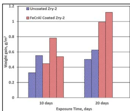
Figure 10. Weight gain of ~1.3 \mu m FeCrAl coated Zircaloy-2 and uncoated Zircaloy-2 in the simulated BWR-NWC for 10 days and 20 days.
