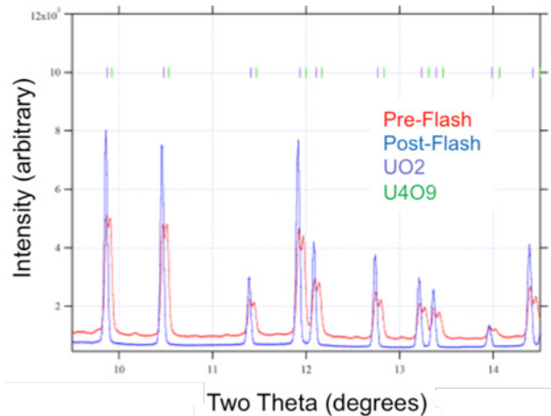
Figure 25. Plot of powder diffraction pattern before the flash and after the flash illustrating the change in phase content with corresponds to the Flash stages.
