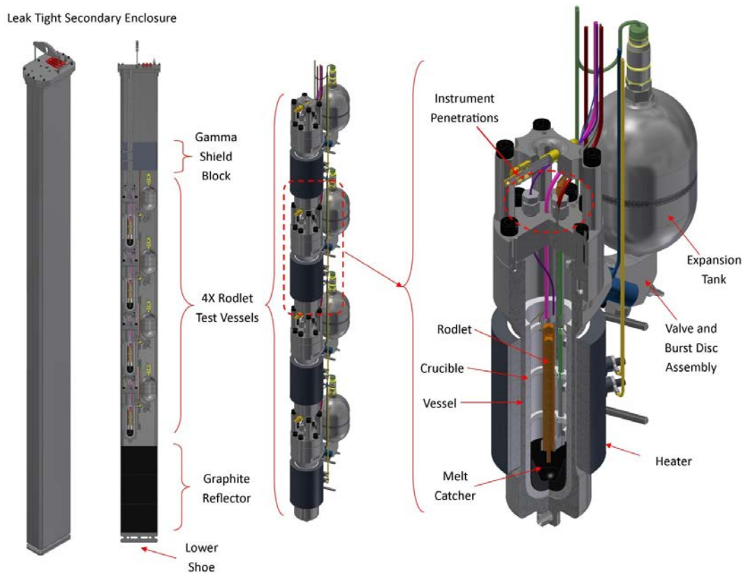
Figure 72. Updated Multi-SERTTA Design
