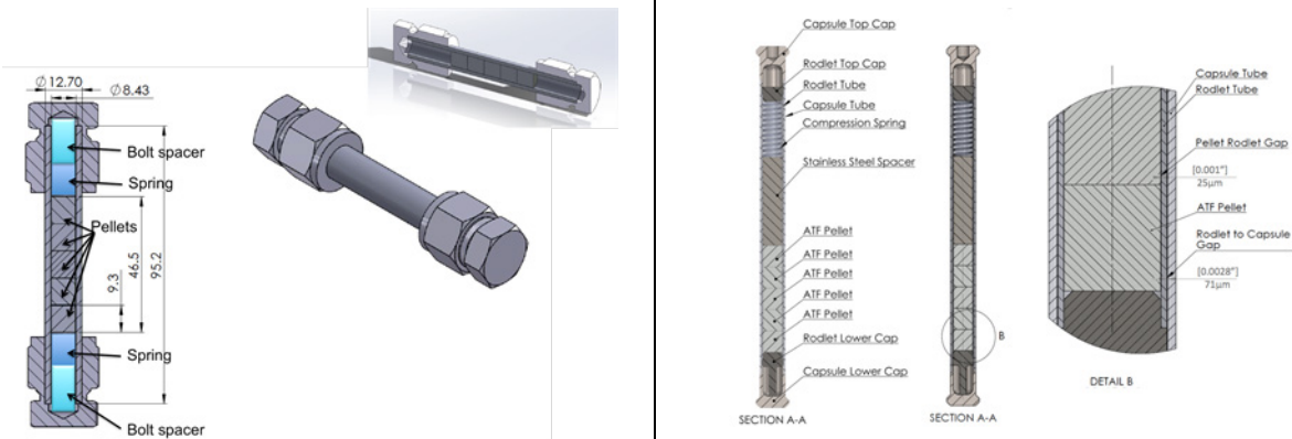
Figure 28. Left image depiction of Swagelok capsule and right image is of ATF-1/LANL-1 rodlet and capsule configuration.
