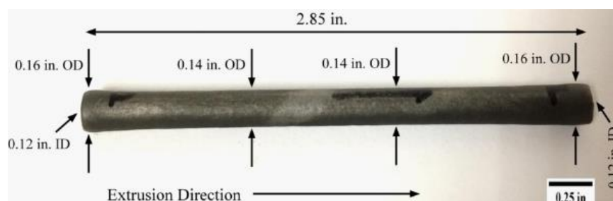
Figure 101. The FCRD-NFA1 tube was produced by hydrostatic extrusion at Case Western Reserve University.
