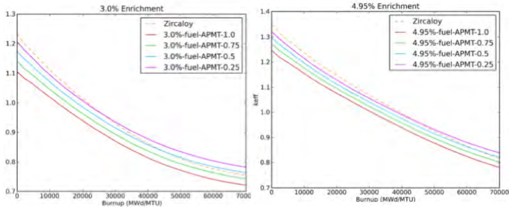
Figure 16. Enrichment Reactivity vs Burnup (MWd/MTU)
