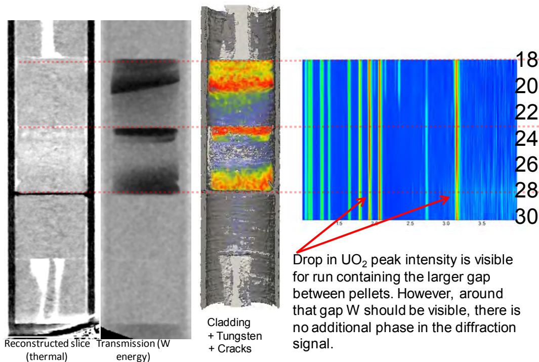
Figure 80. Neutron imaging and diffraction on dUO 2 rodlet containing microstructure and void pellets.
