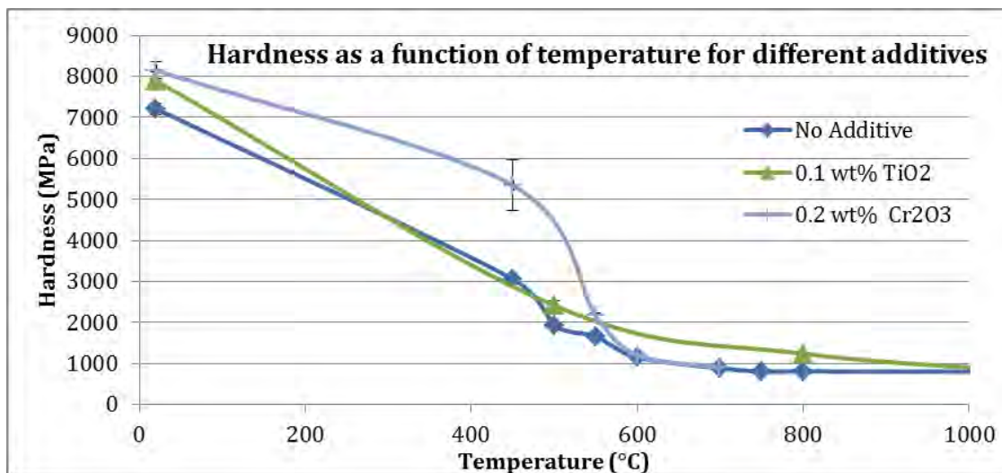
Figure 25. Vickers hardness for the 0.1 wt% \text{TiO}_2 -doped and 0.2 wt% \text{Cr}_2\text{O}_3 -doped samples. The other additives types did not cause substantial changes in hardness.
