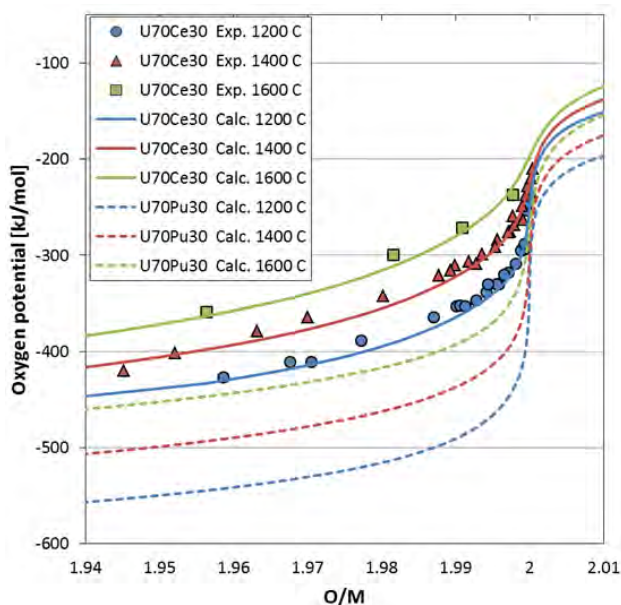
Figure 23. Oxygen potential – O/M ratio developed for U70Ce30 and U70Pu30 analyzed by defect chemistry based on the experimental results by gas equilibrium method.
