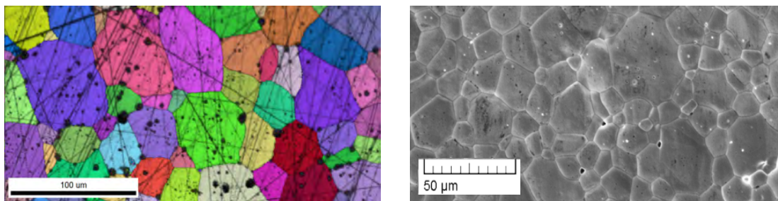
Figure 24. A) OIM map of a 0.2 wt% \text{TiO}_2 -doped sample. B) Bi-modal microstructure seen in a 0.2 wt% \text{Cr}_2\text{O}_3 -doped sample.
