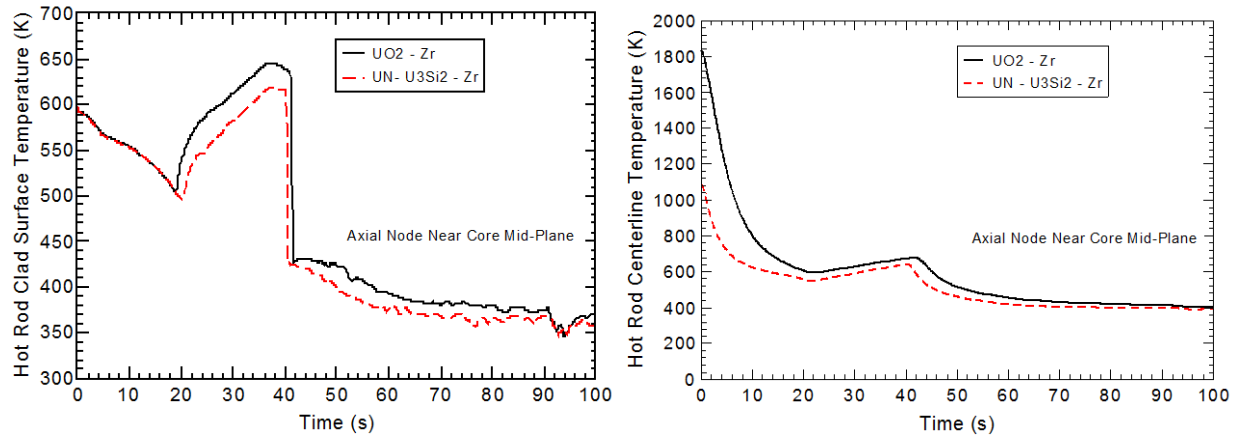
Figure 12. Hot rod clad surface temperature (left) and hot rod centerline temperature for LB-LOCA event in \text{UO}_2 and \text{UN-U}_3\text{Si}_2 fuelled PWRs.
