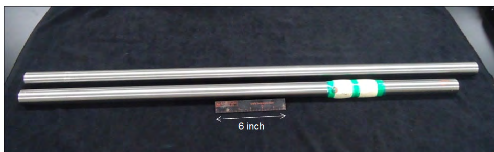
Figure 39. Machined master tubes at Rhenium Alloys, Inc. prior to tube drawing process.
