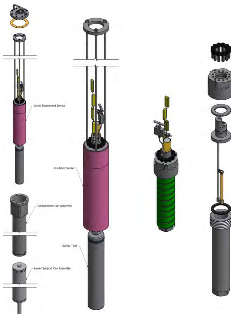
Figure 83. TREAT test loop for ATF fuel testing.
