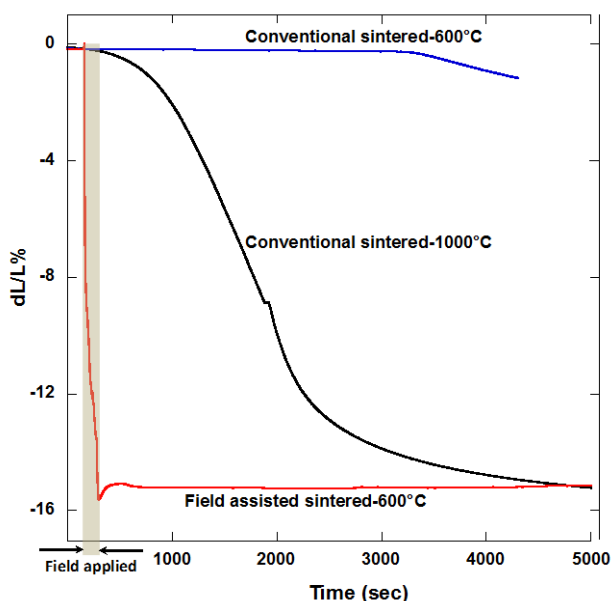
Figure 27. Sintering strain ( dL/L_0\% ) obtained from \text{UO}_{2.16} comparing FAS sintering at 600°C conventional sintering at 600°C and 1000°C.
