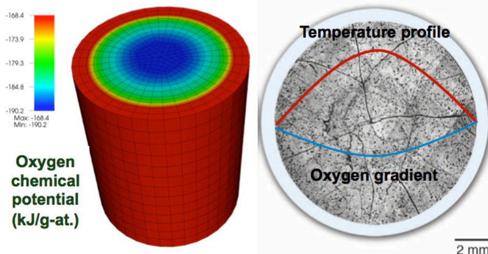
Figure 8. Oxygen Distribution in Irradiated Fuel Pellet
