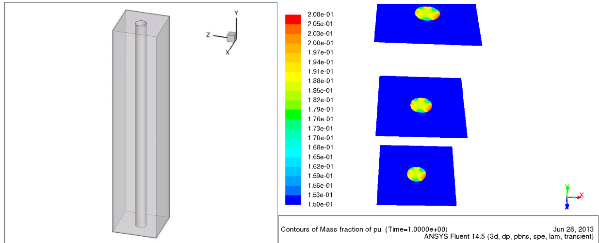
Figure 53. Simple fuel rod geometry and preliminary U-Pu segregation simulation results.
