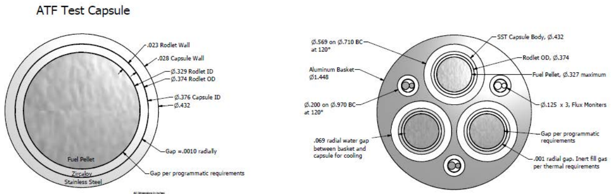
Figure 24. ATF-1 Experiment Component Cross Sections.
