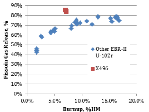
Figure 41. Fission gas release from X496 pins compared to higher smeared density (75%) U-10Zr irradiations in EBR-II.
