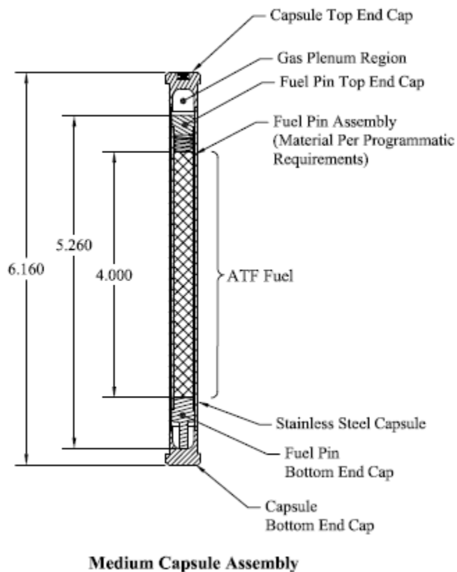
Figure 25. ATF-1 Capsule and Rodlet Design
