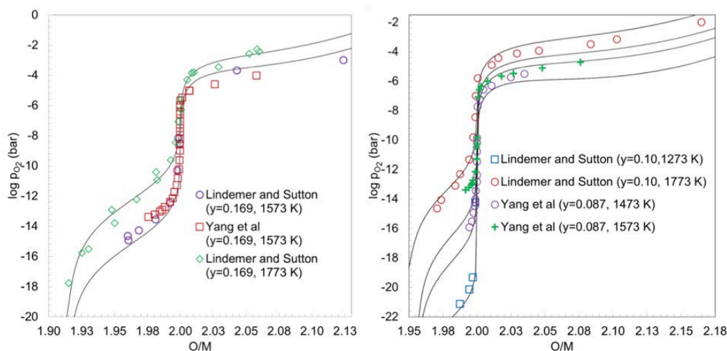
Figure 9. Calculated versus experimental oxygen pressures in \text{U}_{1-y}\text{Gd}_y\text{O}_{2\pm x}
