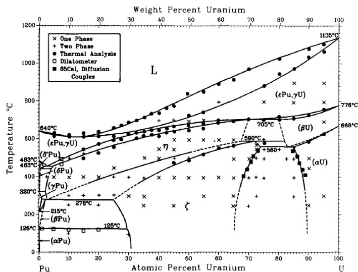
Figure 52. Phase diagram representations for simple, linear alloys, and complex uranium-plutonium alloys.
