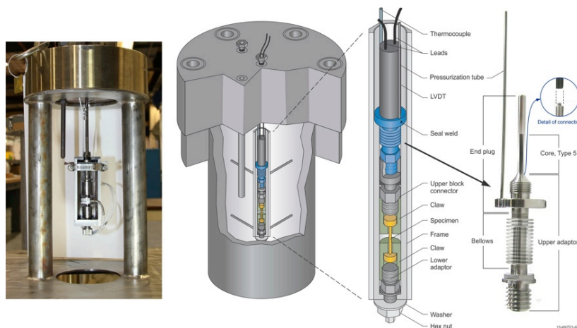
Figure 54. New variable load creep test rig now available.
