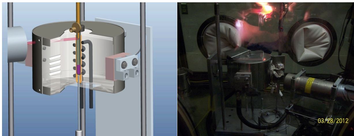
Figure 27. Left: design drawing of the Americium Distillation Furnace including tantalum tube (olive color) containing molten Americium (plum color) and special gamma detector (upper left of picture). Right: actual Americium Distillation Furnace assembled in glovebox showing the special gamma detector (tube with yellow tape at right) that accurately measures movement of radioactive metal from hot distillation zone to cold condensation zone.
