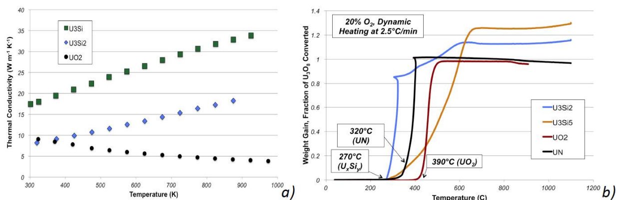
Figure 11. (a) Thermal conductivity of U 3 Si and U 3 Si 2 as a function of temperature compared to that of UO 2 . (b) Oxidation of U 3 Si 2 and U 3 Si 5 in synthetic air compared to UN and UO 2 .
