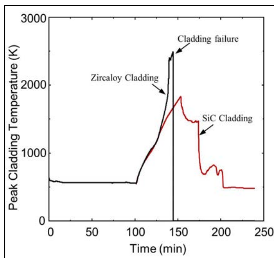
Figure 22. Comparison of MELCOR-predicted maximum cladding temperature during a TMI-2 accident sequence for Zircaloy and SiC cladding and structural components.
