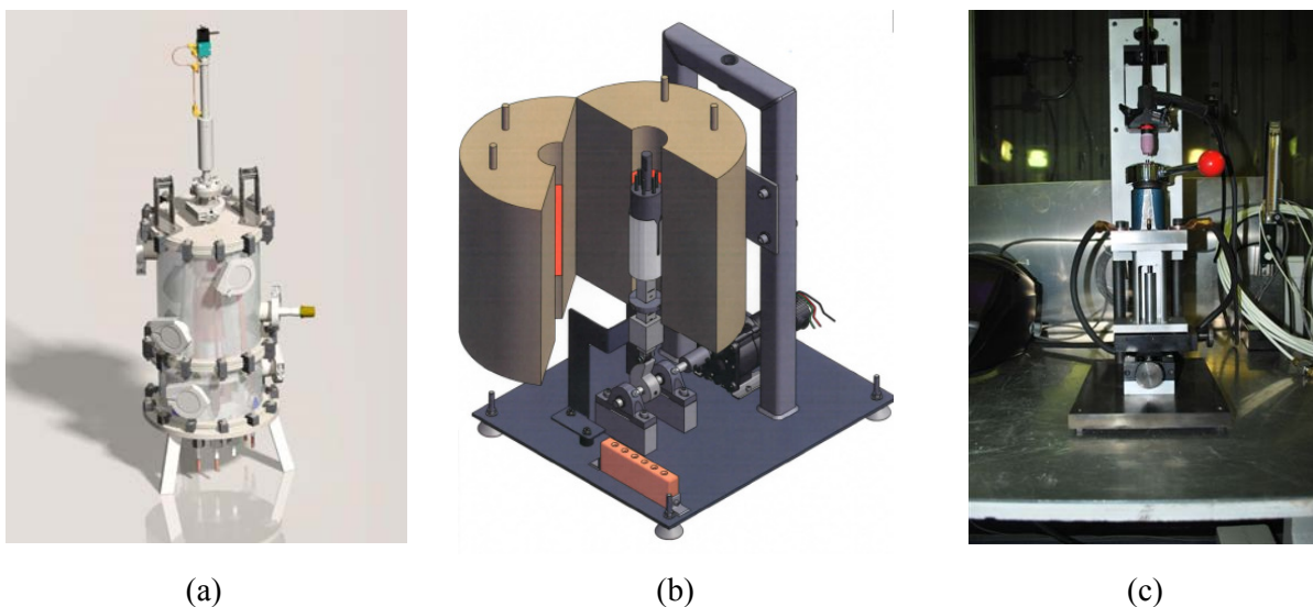
Figure 4. (a) Design model of JFCS casting furnace. (b) Design model of the settler/bonder. (c) Mock-up developmental welding system.
